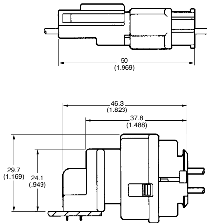
Connector Profile (Ref.)
